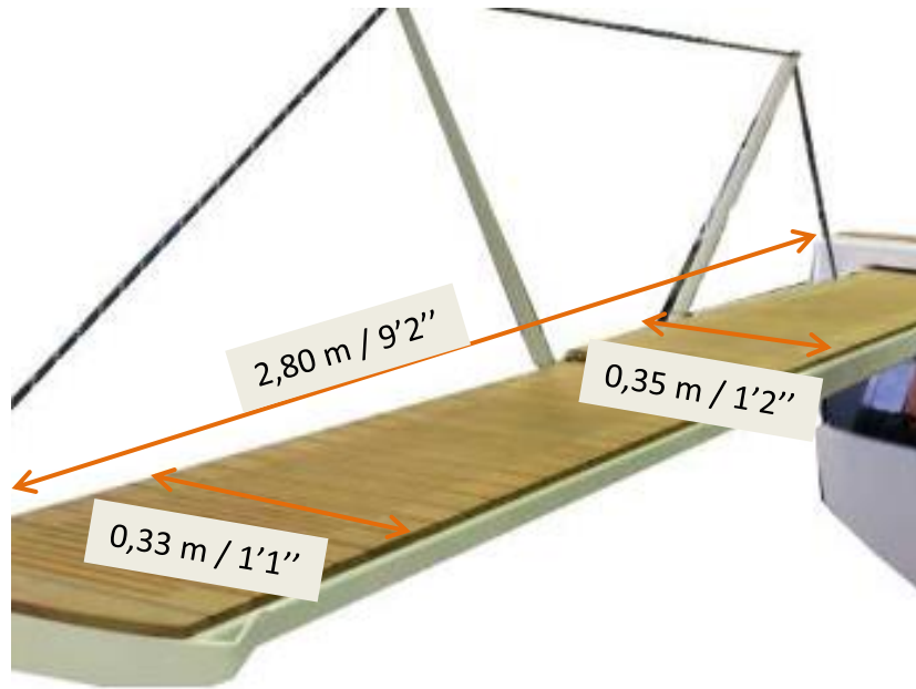
Charge max / Max load: 100 kg / 220 lbs
