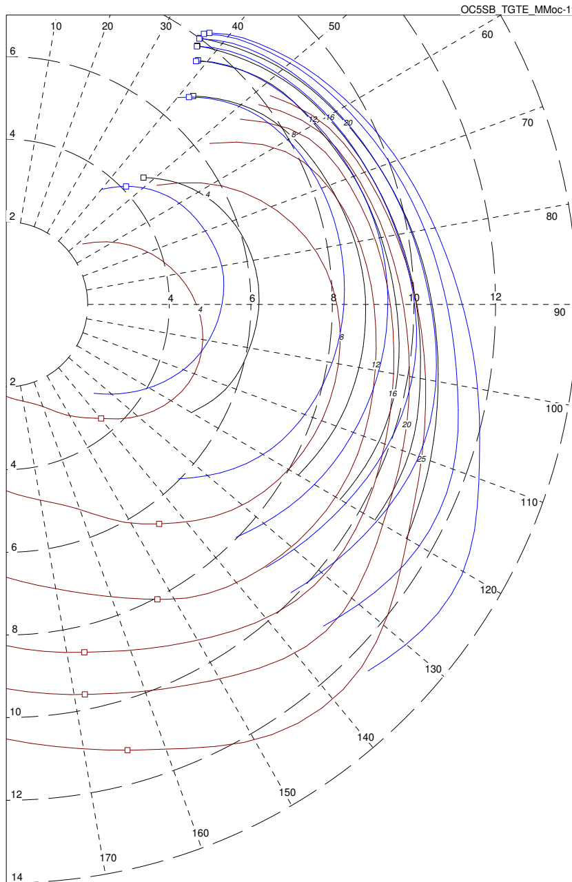
T:\BATEAUX_Developpement\OC5SB N°42\Analyse\8 VPP\VPP 19 06 2017\OC5SB_TGTE_MMoc-19.06.17.vpp 09/07/17 11:45:54 Wind values at 10 m. height.
